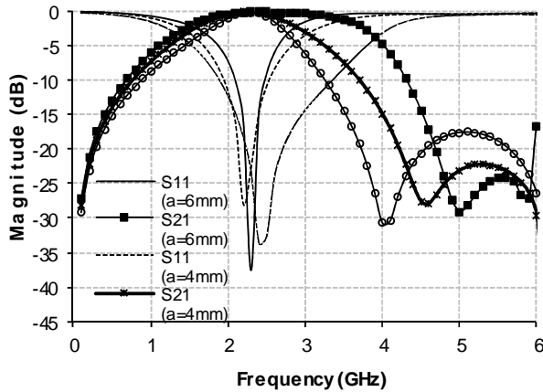
Fig.5. S11 and S21 for different values of conductor length, 'a'
