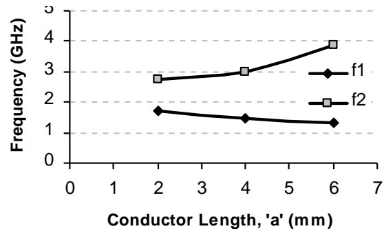
Fig.6(b) Variation of 'f1 & f2' with 'a'
