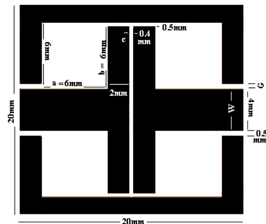
Fig.1(a) schematic diagram
