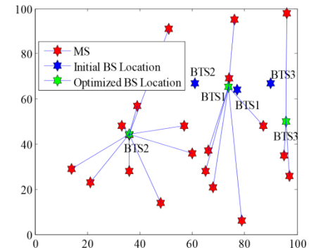
Figure 5: Optimized locations of all three base stations searched by SITO
