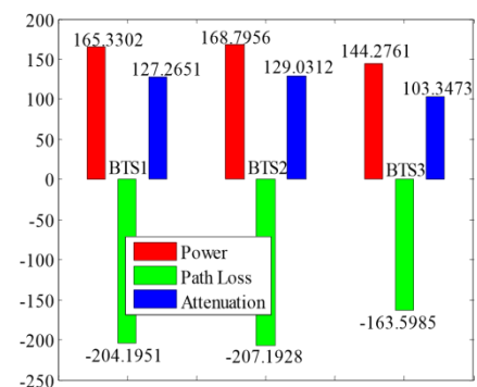
Figure 6: Power Received, Path loss, and Attenuation for all three BS locations searched by PSO
