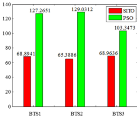
Figure 10: Attenuation comparison for all three BS locations
