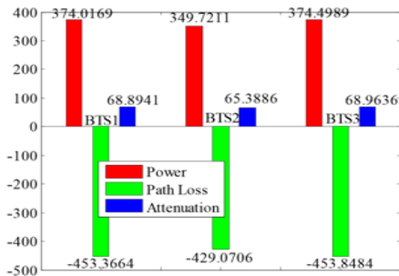
Figure 7: Power Received, Path loss, and Attenuation for all three BS locations searched by SITO
