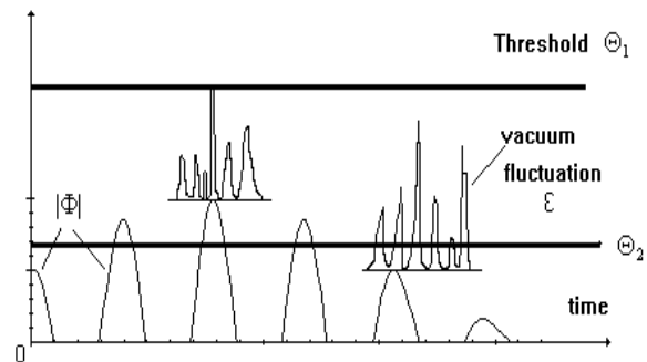
Fig.4. Quantum measurements.
