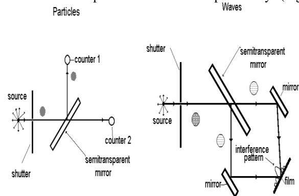
Fig.1. Experiments with individual photons on semitransparent mirror.
