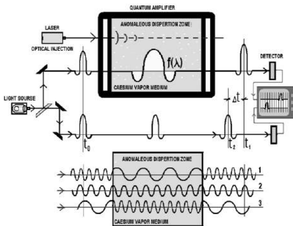
Fig. 5. Experiments of L.Wang - superluminal light propagation.
