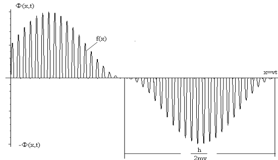
Fig. 2. Behaviour of wave packet in linear dispersion medium (i.e., rather like a series of stroboscopic photographs).
